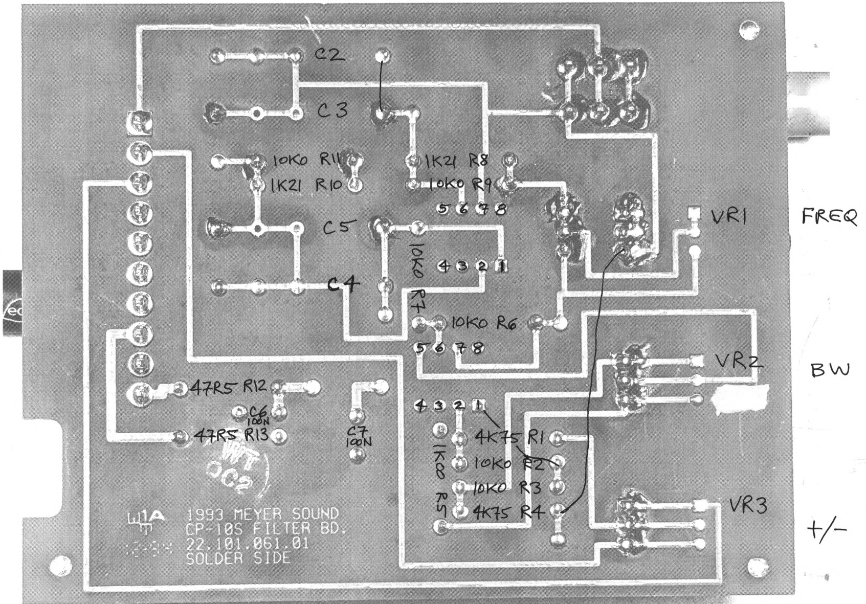
MEYER CP10 FILTER BOARD
