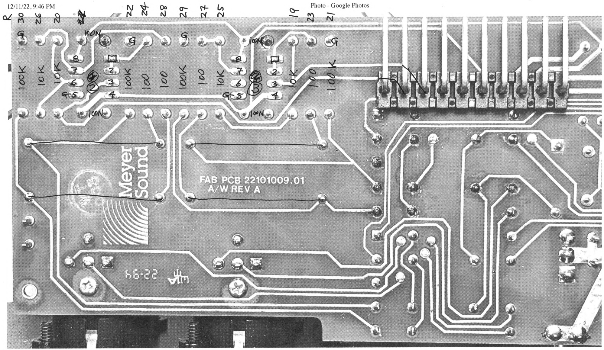
MEYER CP10 I/O BOARD OUTPUT AMPS
