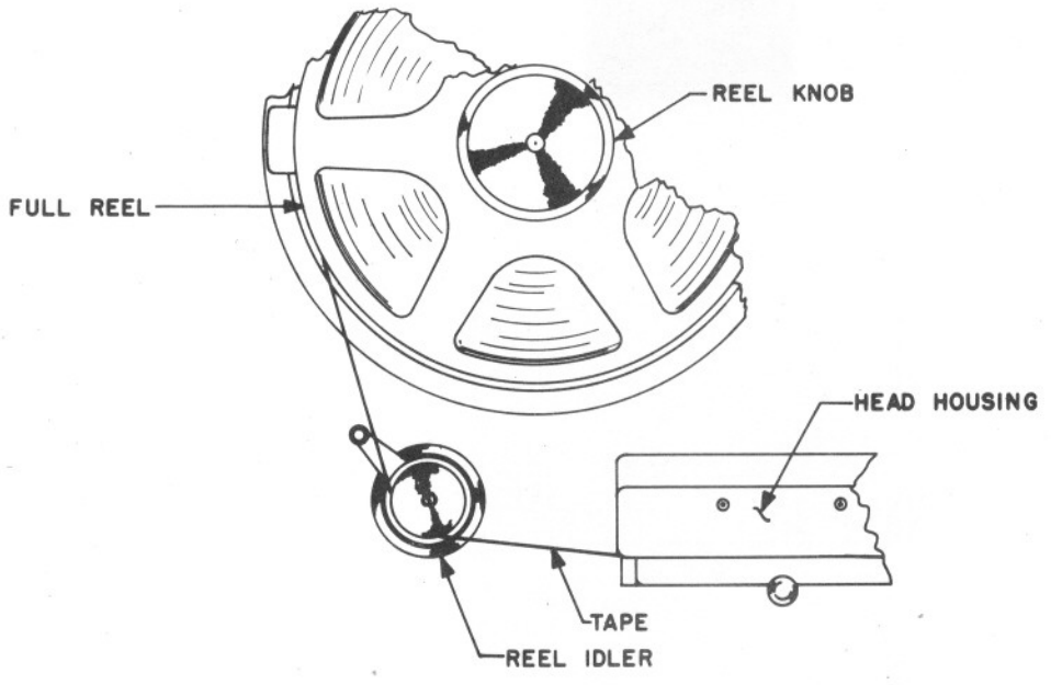
REEL IDLER ASSEMBLY SERIES 300 AMPEX ELECTRIC CORPORATION REDWOOD CITY, CALIFORNIA
