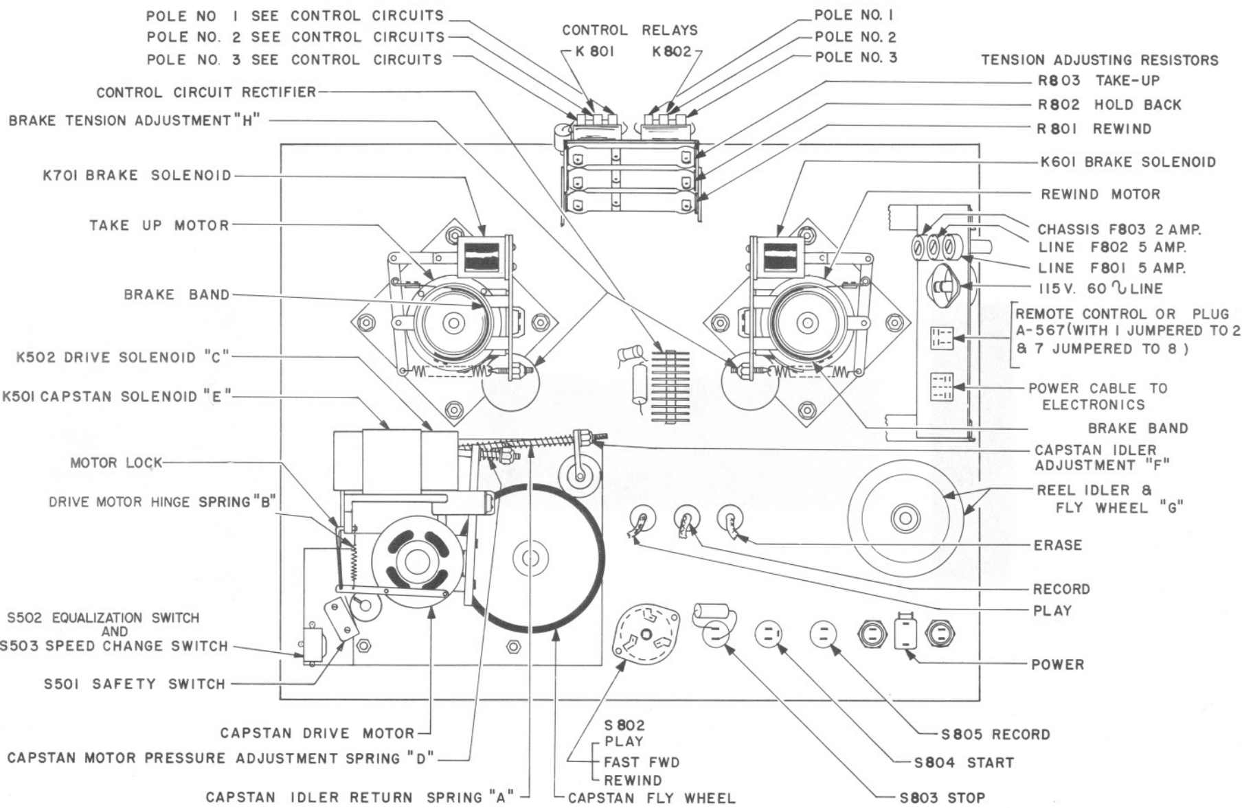
TOP PLATE ASSEMBLY (BOTTOM VIEW)
