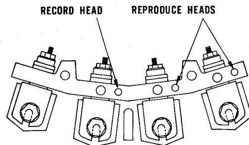
Fig. 5-2 Head Azimuth Adjustment Points
