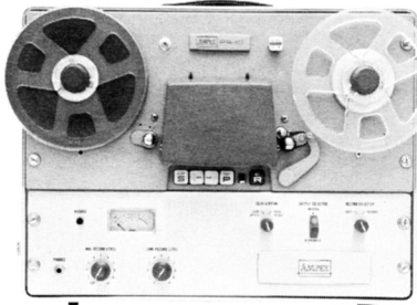
Model PR-10-1 Portable
