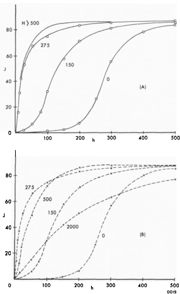
Anhyysteretic intensity of magnetization (J) is plotted against the unidirectional field strength (h) for various amplitudes of a-c bias in this chart. In (A) the bias field was reduced while holding the unidirectional field constant. In (B) both fields were reduced simultaneously. Note in (B) that increasing the bias field beyond a certain value decreases the intensity of magnetization.
