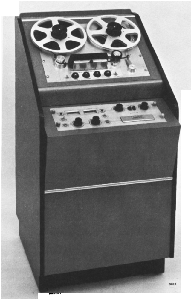
A console mounted Ampex Model 354, two channel recorder/reproducer.
