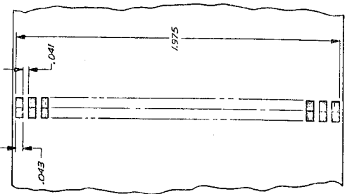
24 TRACK .043 TRACKS ON .084 CENTERS
