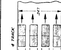
1/4 TRACK & 4 TRACK .043 TRACK ON .136 CENTERS IN ONE HEAD STACK TAPE TRACKS IDENTICAL
