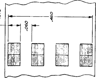
1/2" TAPE (.500/.496) 4 TRACK .070 TRACKS ON .130 CENTERS
