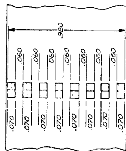
1" TAPE (1.000/.996) SCALE: 3/4" 8 TRACK .070 TRACKS ON .130 CENTERS
