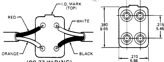
(CC-77 WIRING)
